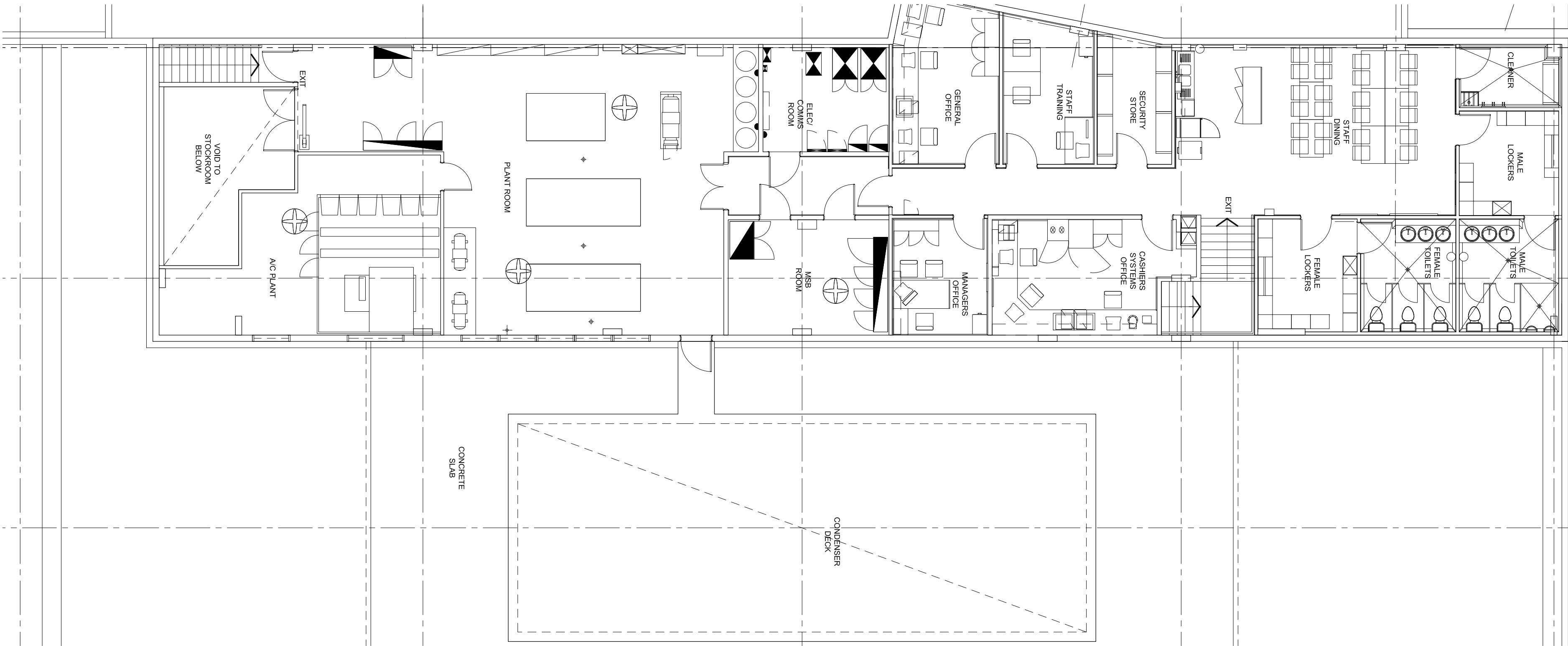
2 MEZZANINE FLOOR - INTERNAL LAYOUT
